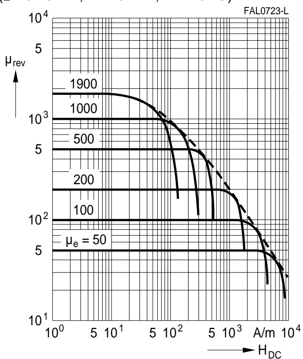
DC magnetic bias of P and RM cores ( \hat{B} \leq 0.25 \text{ mT} , f = 10 \text{ kHz} , T = 25 \text{ }^\circ\text{C} )
